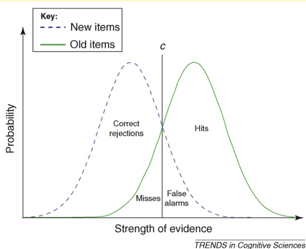
Figure 1. Standard SDT of old and new recognition judgments. c represents the decision criterion. Items to the right of c will be judged old, and those to the left of c will be judged new. An old item is classified as a hit if judged old, or a miss if judged new; a new item is classified as a false alarm if judged old, or a correct rejection if judged new.
